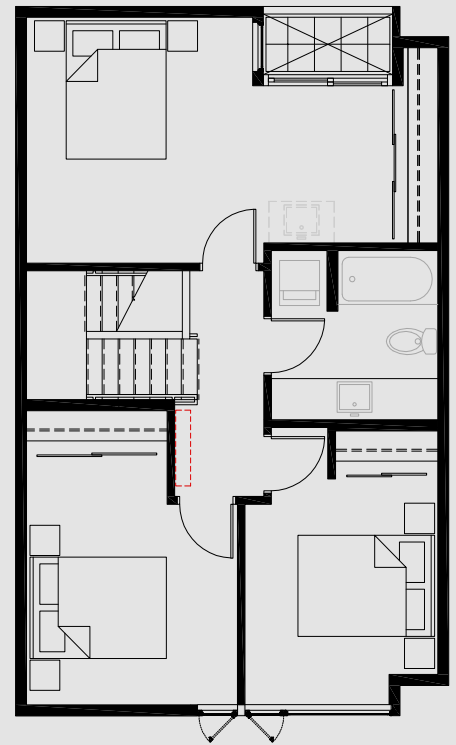
3RD FLOOR
