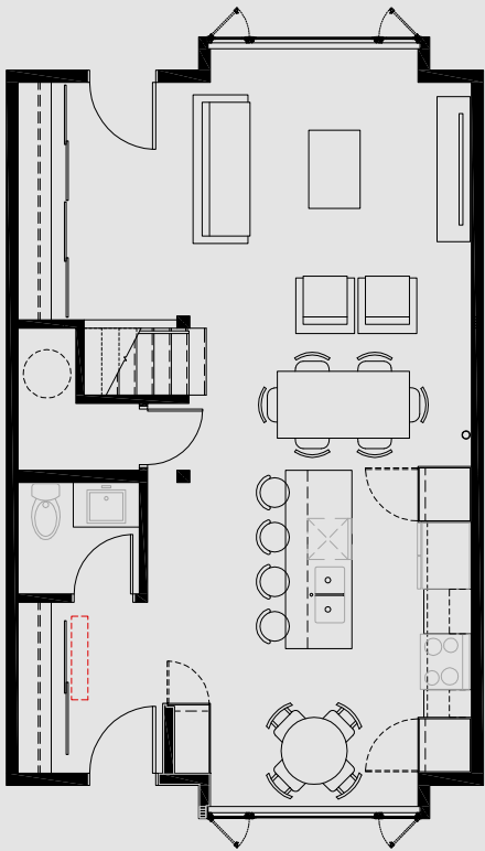
1ST FLOOR
